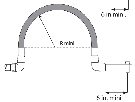
> Expansion loop
