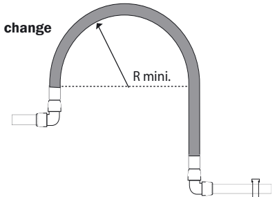
> Obstacle bypass
